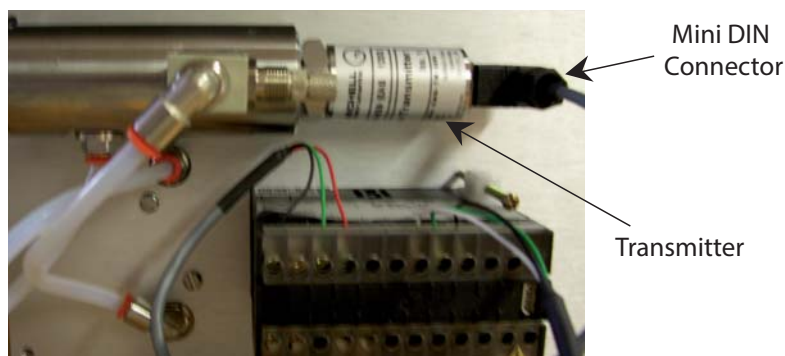
Figure 15 Sensor Removal
